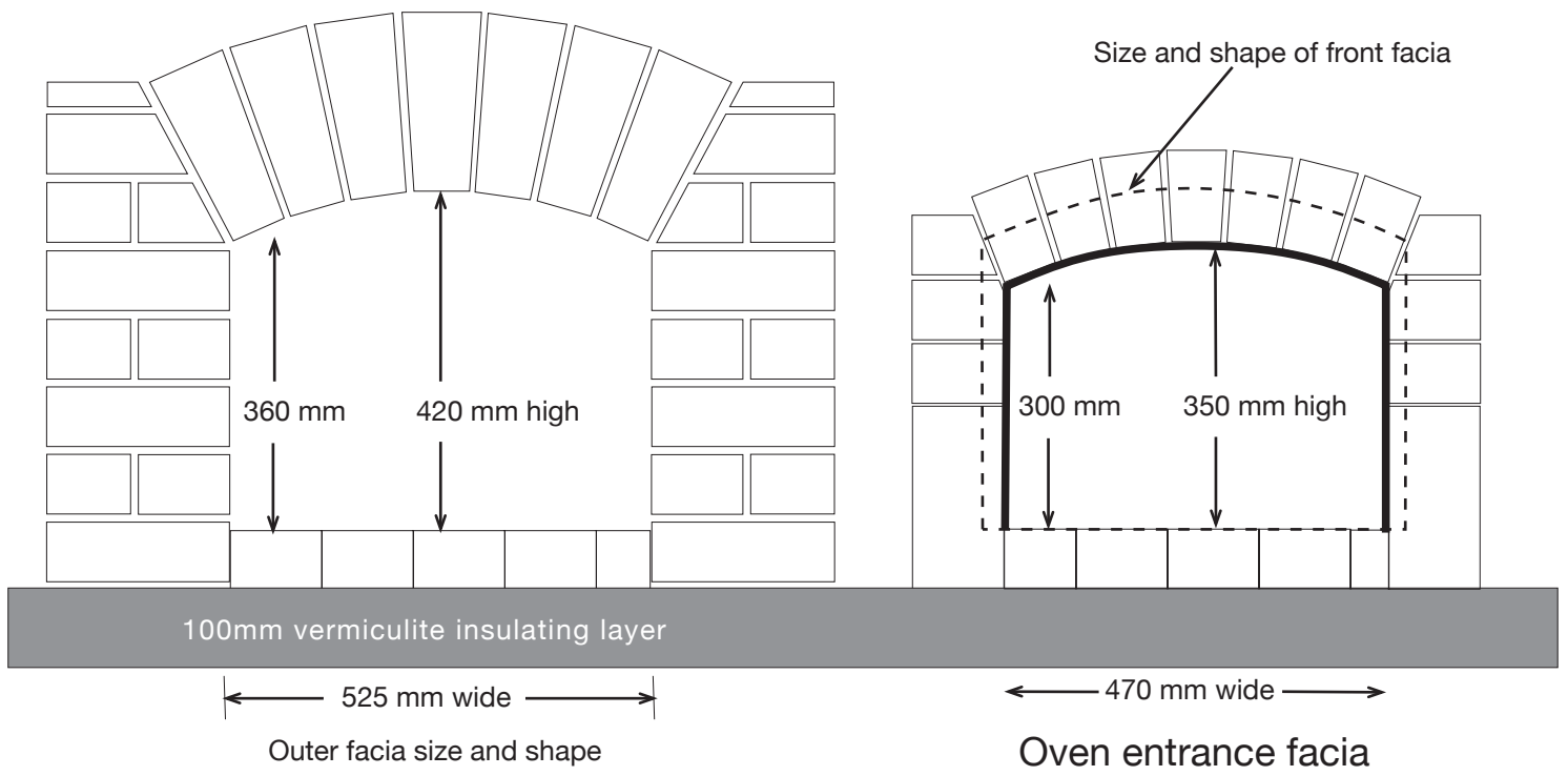
Neill's Pompeii oven facia
