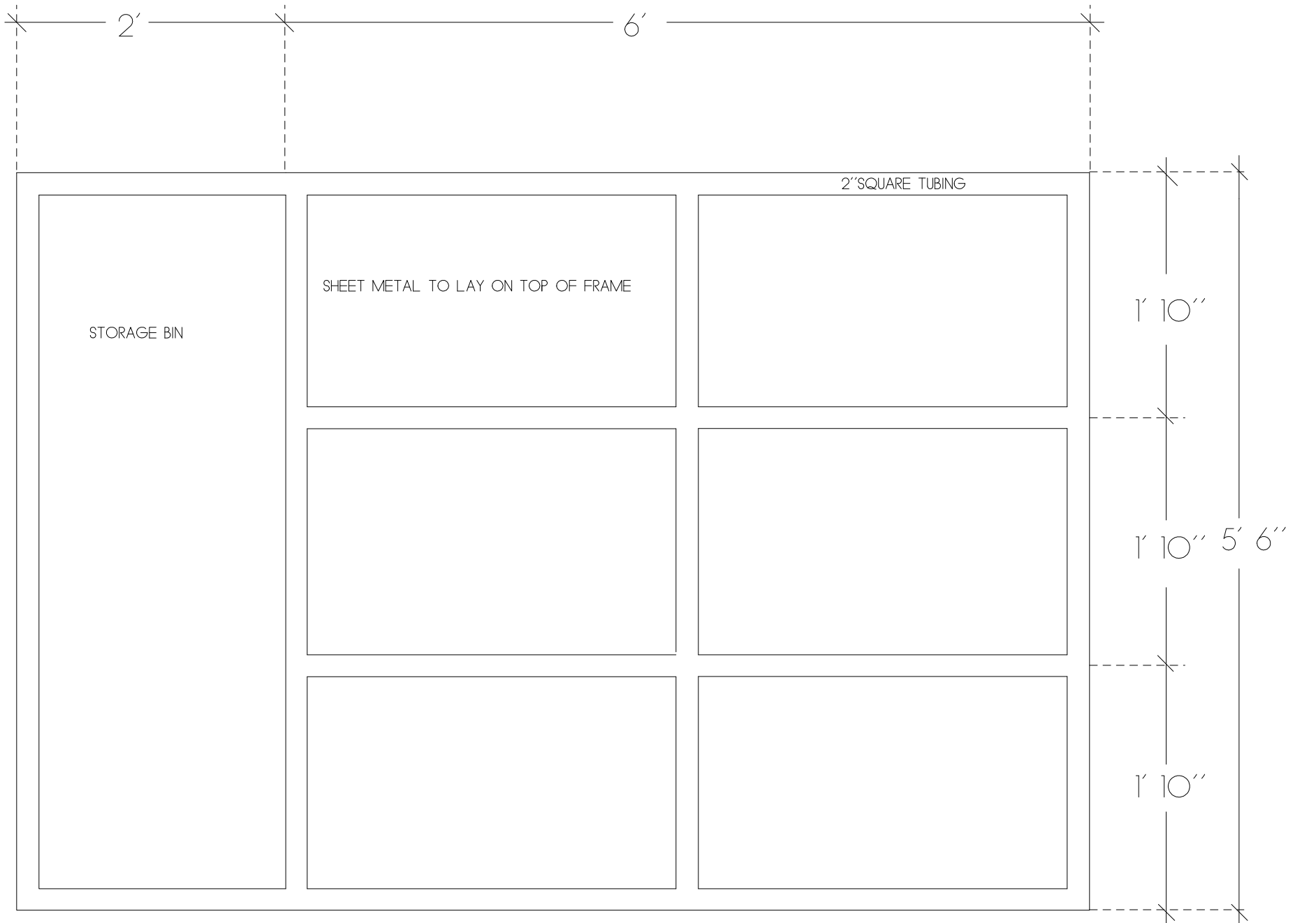
TOPVIEW OF TRAILER BED
