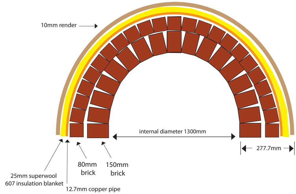
Design B cross section of dome walls
