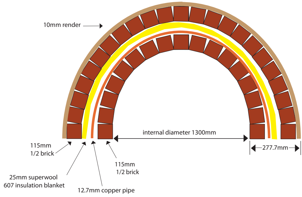
Design A cross section of dome walls
