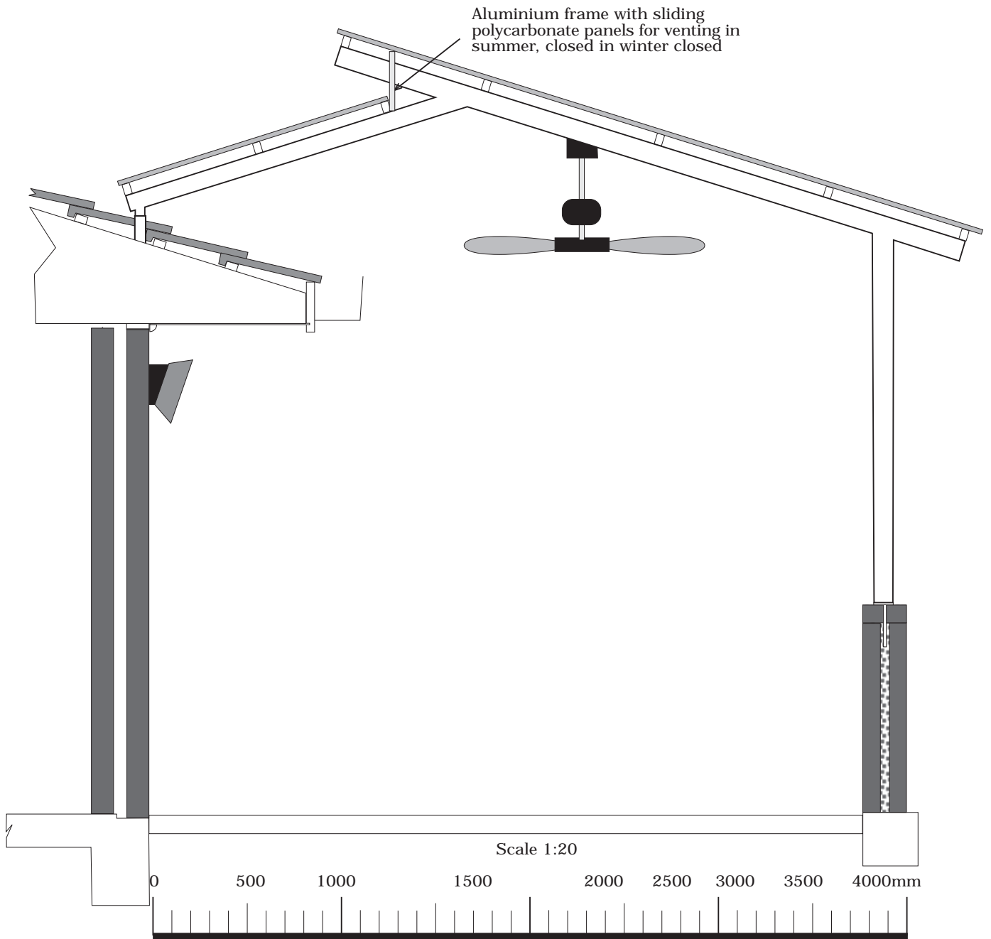
Cross section of patio 3.8 x 13metres
