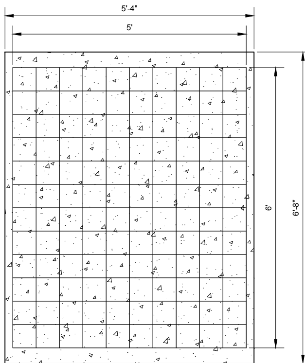
3.5" CONCRETE HEARTH REMESH LAYOUT
