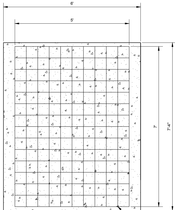
6" CONCRETE BASE REMESH LAYOUT
