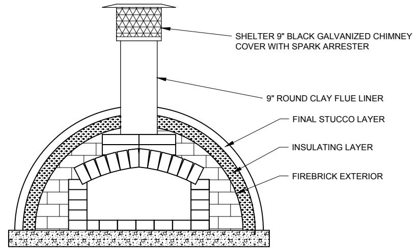
42" INSIDE DIAMETER PIZZA OVEN ON INSULATING HEARTH
