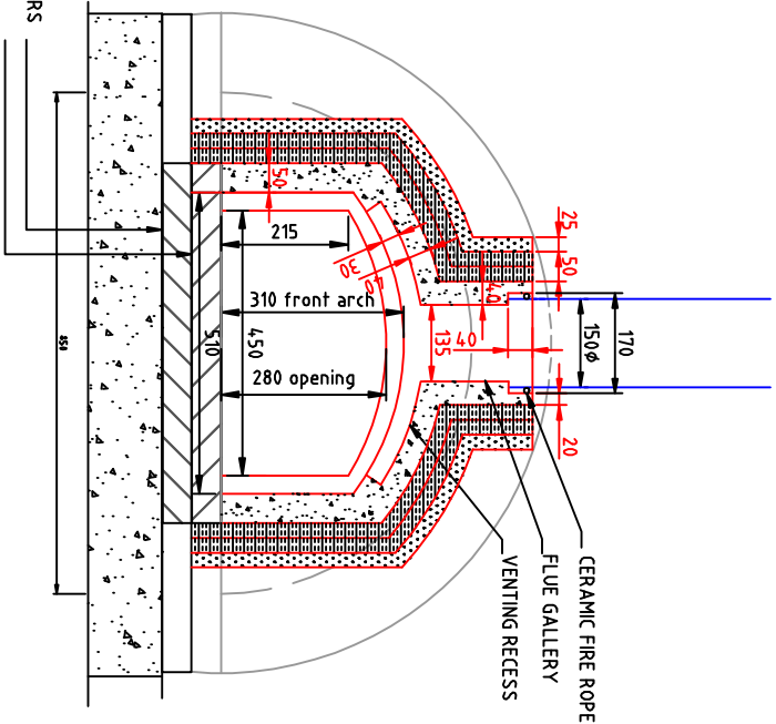
SECTIONAL FRONT ELEVATION
