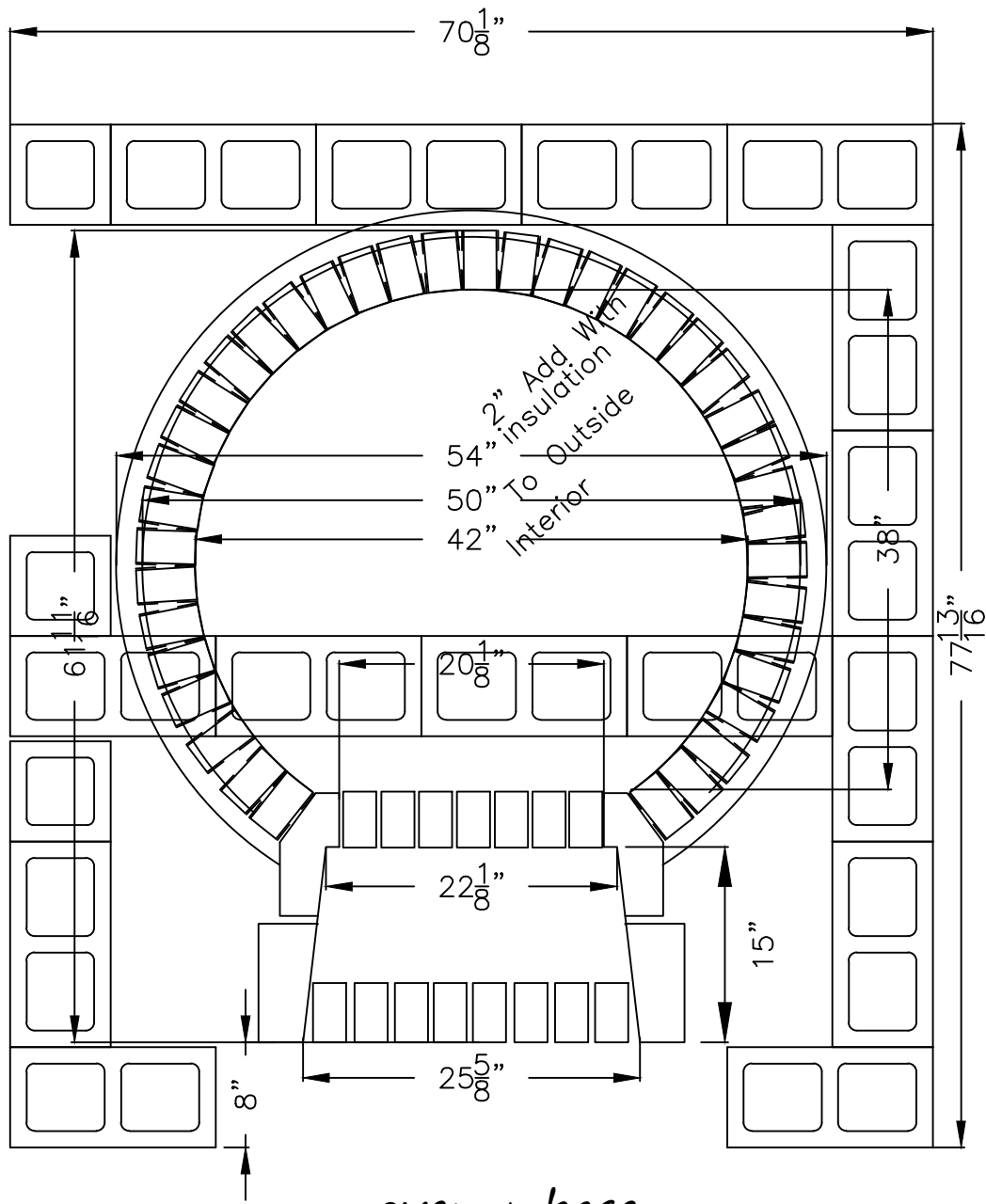
oven + base
