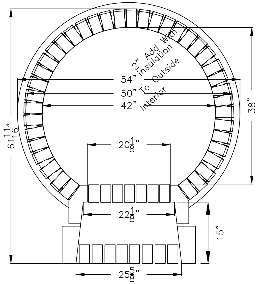
oven
